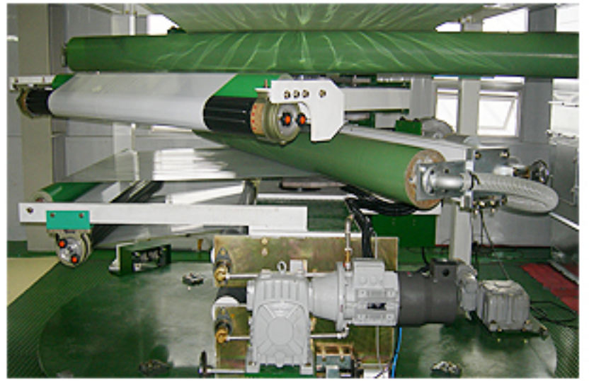
▶ Take-Up Oscillating Unit
